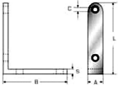
EY08076A S/S AISI 304 STAMPED CORNER BRACKET 30X30 (R3S506)
