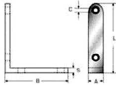
EY08076C S/S AISI 304 STAMPED CORNER BRACKET 50X50 (R3S508)
