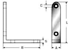
EY08076B S/S AISI 304 STAMPED CORNER BRACKET 40X40 (R3S507)
