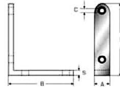
EY08076D S/S AISI 304 STAMPED CORNER BRACKET 60X60 (R3S509)
